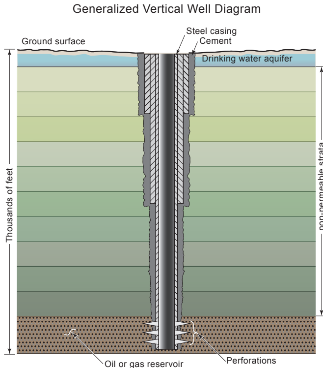
Diagram of a conventional vertical well showing steel casing, cement that bonds the casing to the rocks surrounding the well, and perforations in the casing that allow oil and natural gas to enter the well and be produced. Also shown is a shallow aquifer that supplies drinking water.
