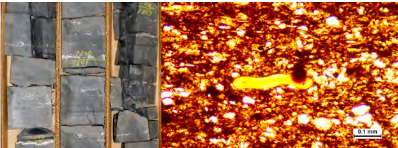
Photograph of a core of a shale reservoir. The inset shows a greatly magnified view of shale. The dark-brown materials are organic remains that when naturally "cooked" will be partially converted to oil and natural gas. The remainder of the rock is mineral matter except for the yellow object, which is a crushed spore. In shales, the pore spaces are too small to be seen even at this very high magnification. Compare to the sandstone core above. Photos by Ron Broadhead.
