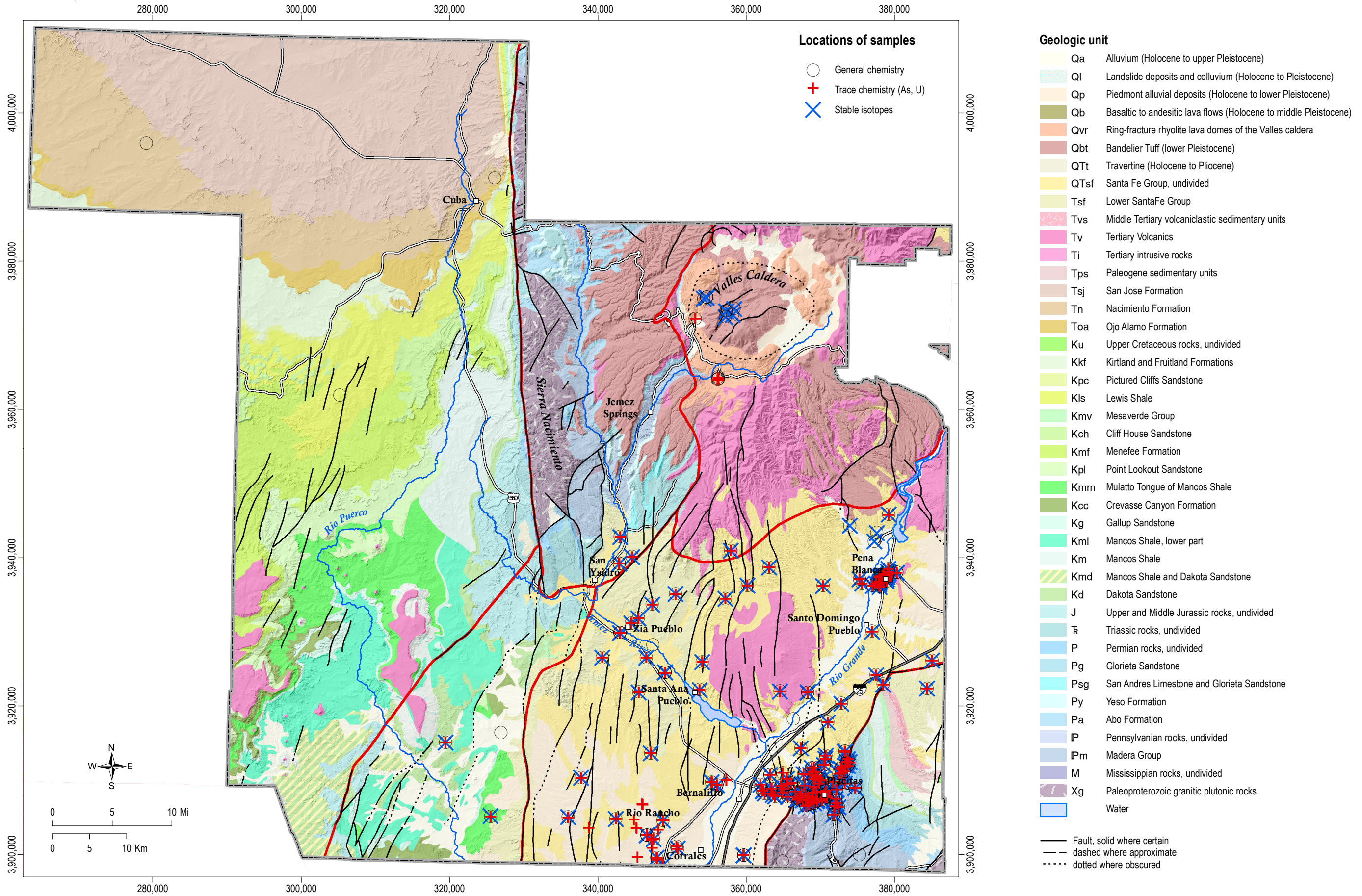
Figure 27. Map of locations of sampled for (o), trace element chemistry (+) and stable isotopes (x). Water chemistry is from NMBGMR Aquifer Mapping Database, and compiled published values and internally measured values from NMBGMR, USGS and other sources.
